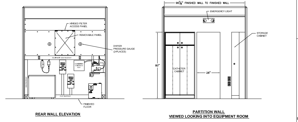
PARTITION WALL VIEWS
